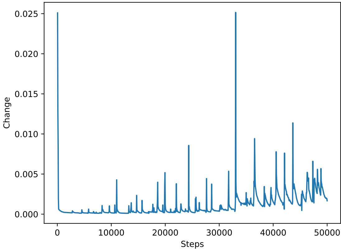
Mean Change in Hamiltonian (simplified)
