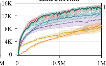
HalfCheetah
