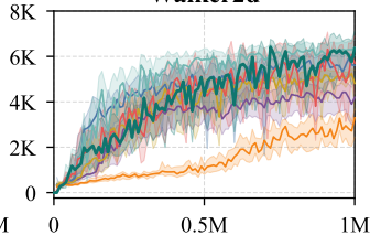
Walker2d
