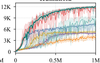
Humanoid
