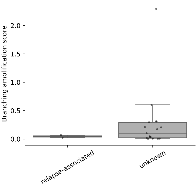
Response status Branching-like amplification by relapse association
