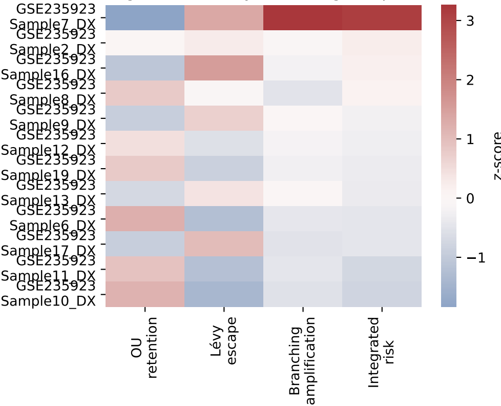
Integrated OU-Lévy-branching risk profile
