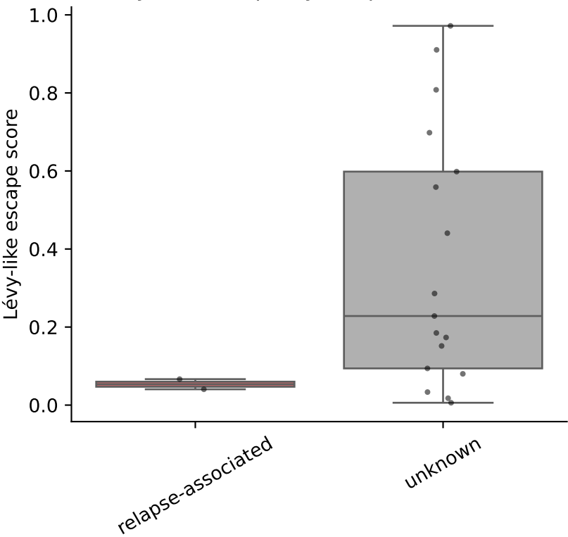
Lévy-like escape by relapse association
