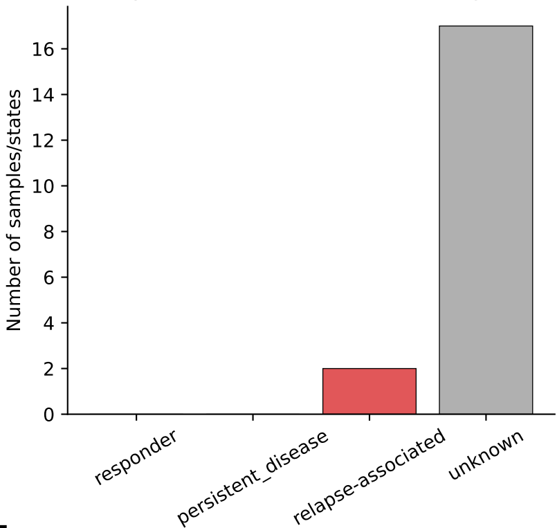
Response status Branching-like amplification by relapse association
