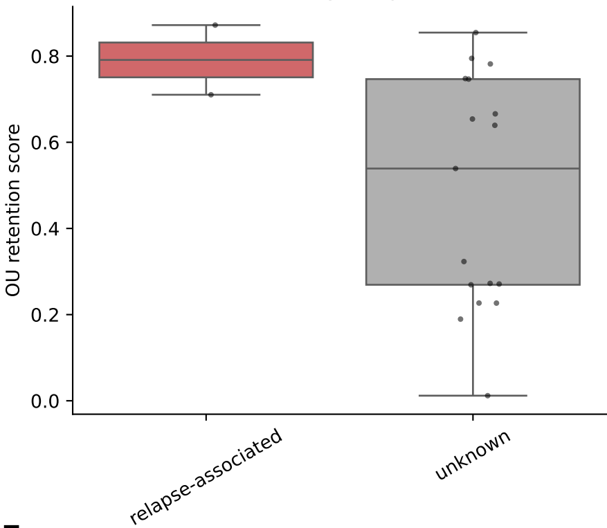
OU-like retention by relapse association
