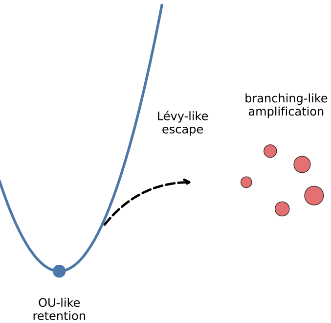
OU-Lévy-branching interpretation
