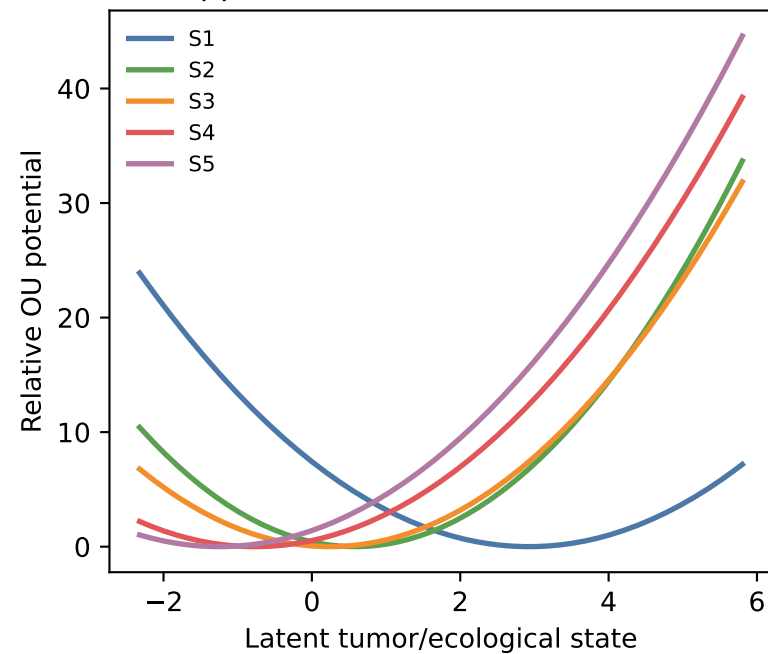
Approximate OU attractor basins
