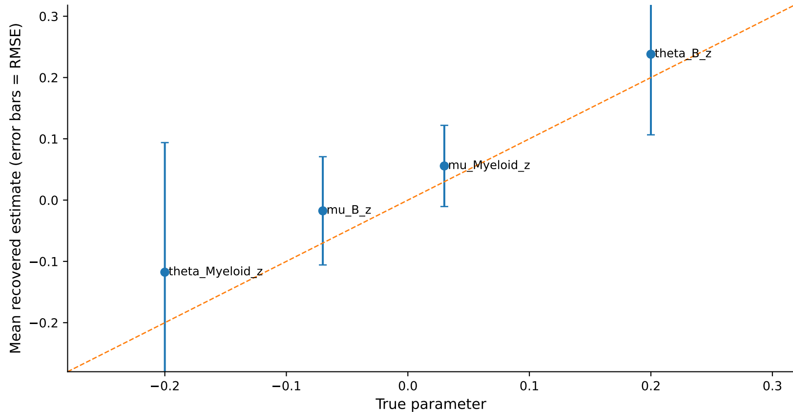
Supplementary Figure S4. Simulation-based parameter recovery
