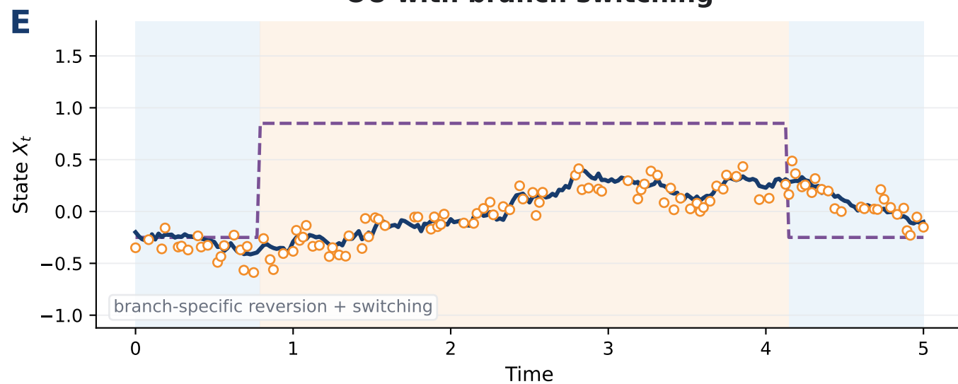
OU with branch switching
