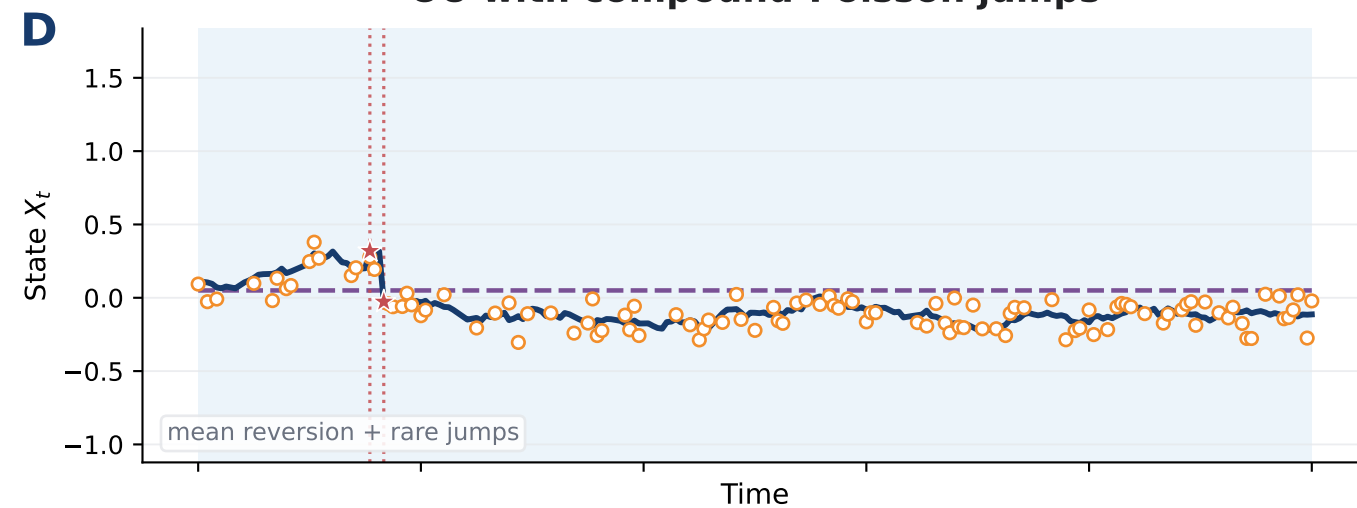
OU with compound-Poisson jumps
