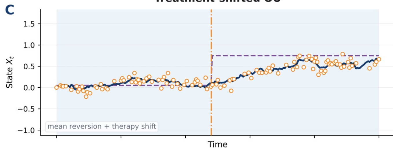
Treatment-shifted OU
