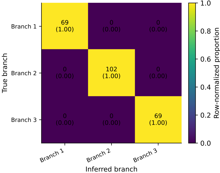
Branch-assignment confusion matrix
