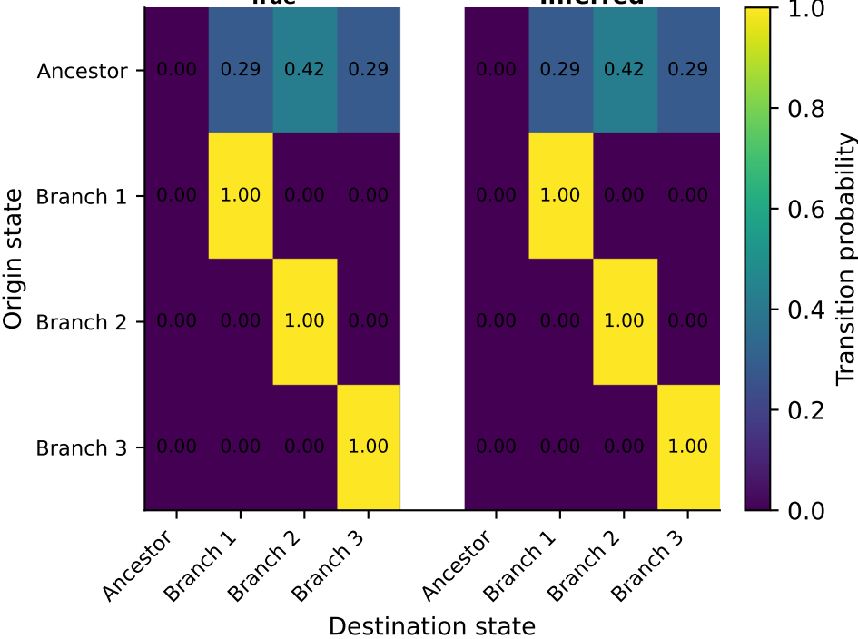
Branch-transition matrix recovery
