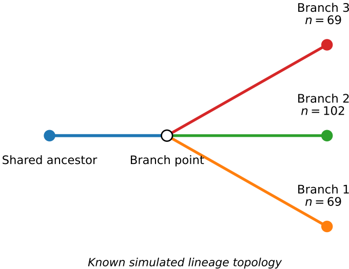
Simulated lineage
