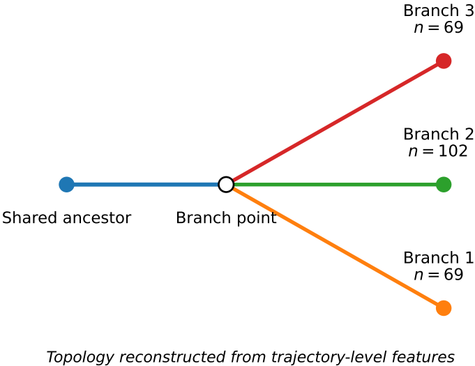
Inferred lineage
