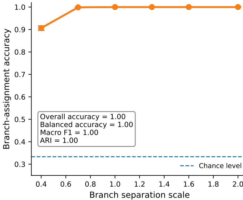
Branch accuracy across separation
