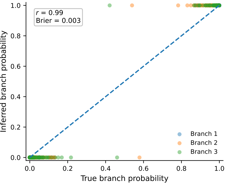
Branch-probability recovery
