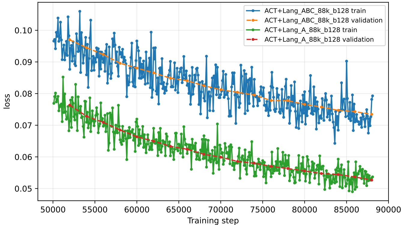
ACT loss
