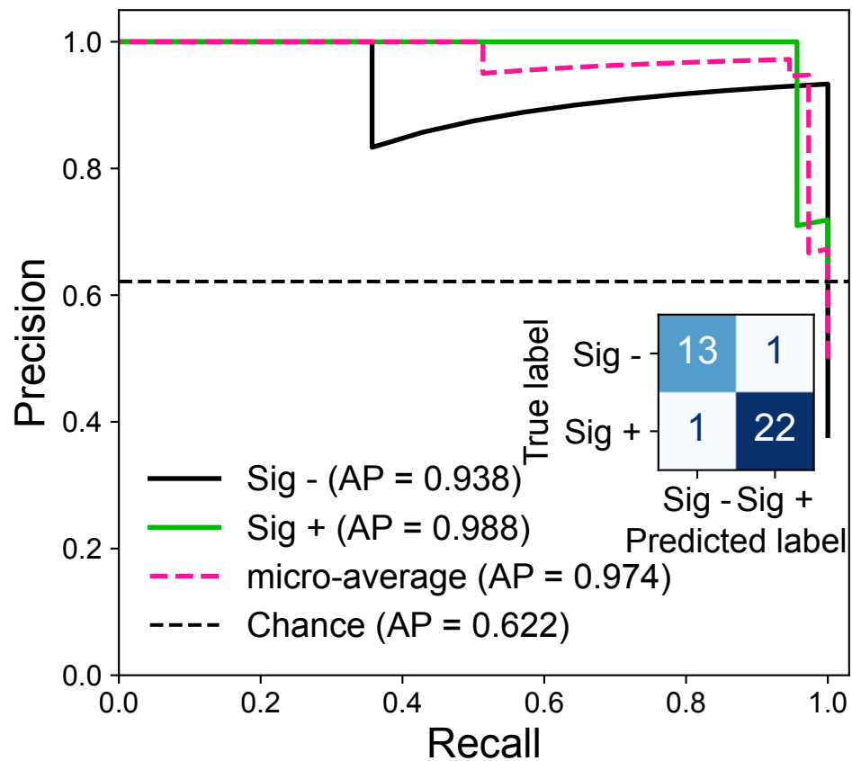
PR Curve
