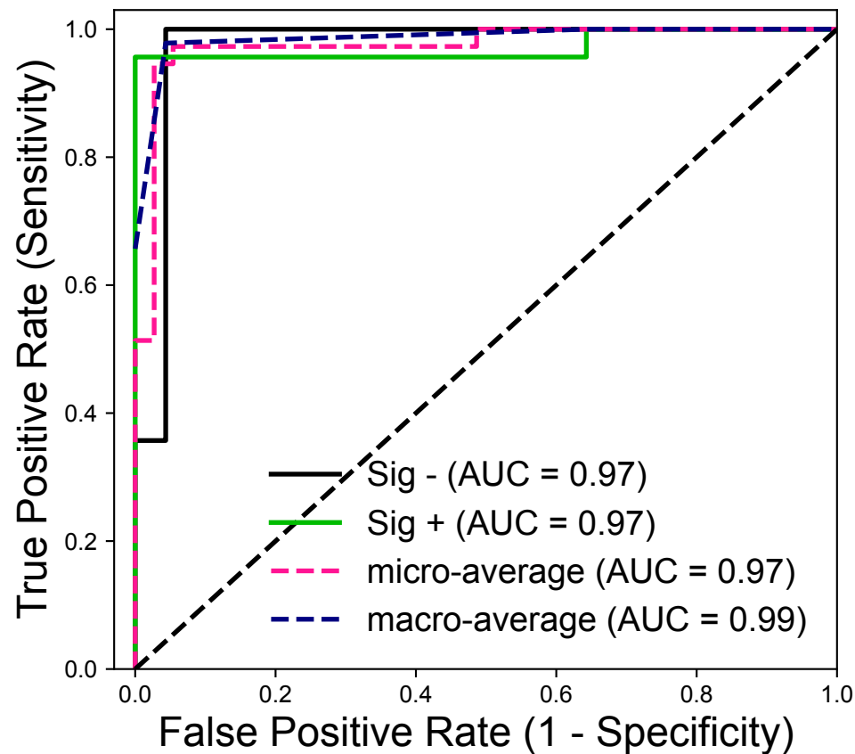
ROC Curve
