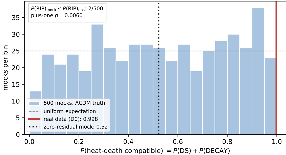
FIG. 3. The completed 500-mock null calibration. Under \Lambda CDM truth the heat-death-compatible posterior mass is consistent with U(0,1) (KS p = 0.154 ) for continuous CPL+P1; the excluded zero-residual diagnostic returns 52/48. Two mocks have P(\text{RIP}) \leq P(\text{RIP})_{\text{obs}} ; the red line marks the observed heat-death-compatible mass.
