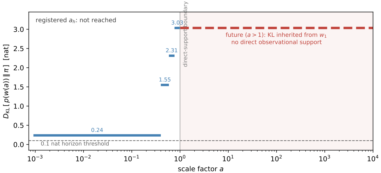
FIG. 7. Constraint horizon (BIN4): posterior-to-prior information in w(a) per bin. The dashed future segment is the w_1 KL inherited by the BIN4 freezing rule, not direct future information. The frozen 0.1-nat threshold is never crossed, so the registered result is a_h : not reached. The vertical line at a = 1 marks the distinct boundary of direct observational support.
