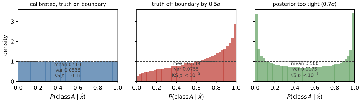
FIG. 8. The boundary-calibration toy (Appendix E). Left: calibrated posterior with the truth on the boundary—class probabilities exactly uniform. Center: truth off the boundary by 0.5\sigma —direction information appears, as it should. Right: over-confident posterior—mean preserved but variance above 1/12 ; the uniformity diagnostics fail precisely when the pipeline is defective.
