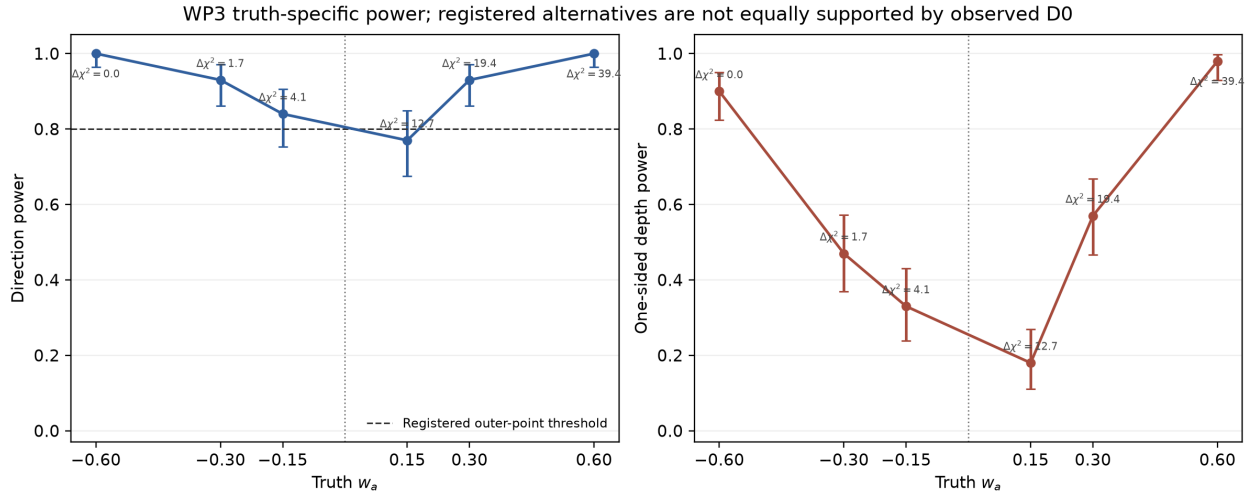
FIG. 4. WP3 direction and one-sided depth power at six registered constrained truths. Error bars are exact 95% binomial intervals; annotations give each truth’s D0 profile \Delta\chi^2 relative to the best registered truth. The unequal profile penalties prevent reading the two sides as equally supported, symmetric effect sizes.
