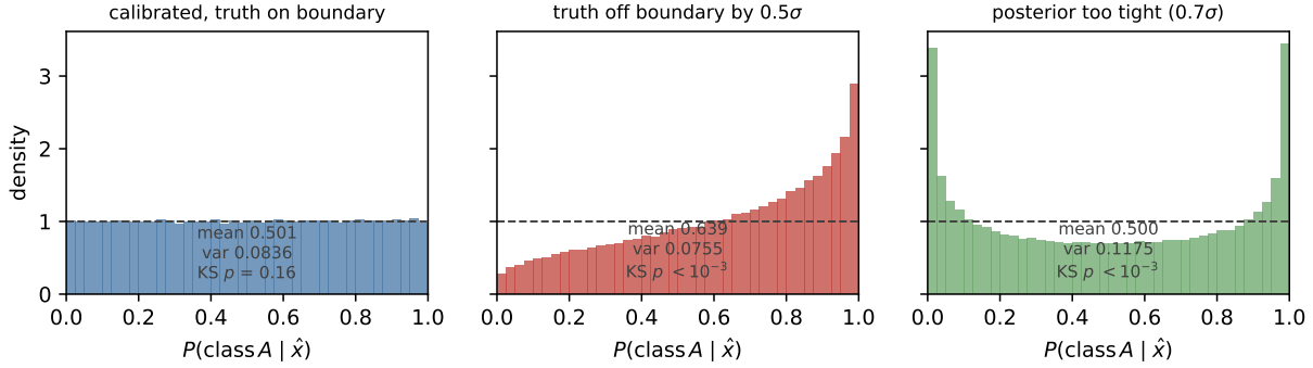
FIG. 7. The boundary-calibration toy (Appendix E). Left: calibrated posterior with the truth on the boundary—class probabilities exactly uniform. Center: truth off the boundary by 0.5\sigma —direction information appears, as it should. Right: over-confident posterior—mean preserved but variance above 1/12 ; the uniformity diagnostics fail precisely when the pipeline is defective.
