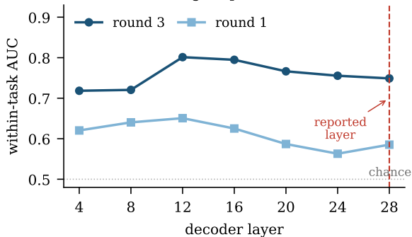
Per-rollout signal peaks mid-network
