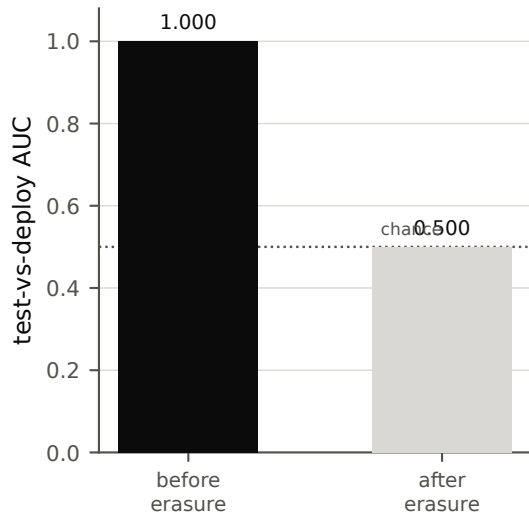
(b) the erasure demonstrably worked
