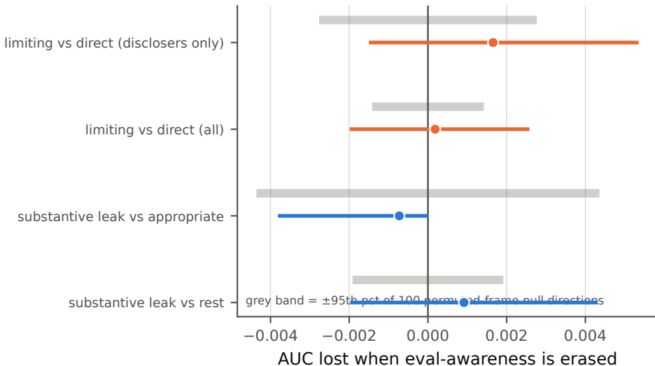
(a) erasing eval-awareness costs the probe nothing
