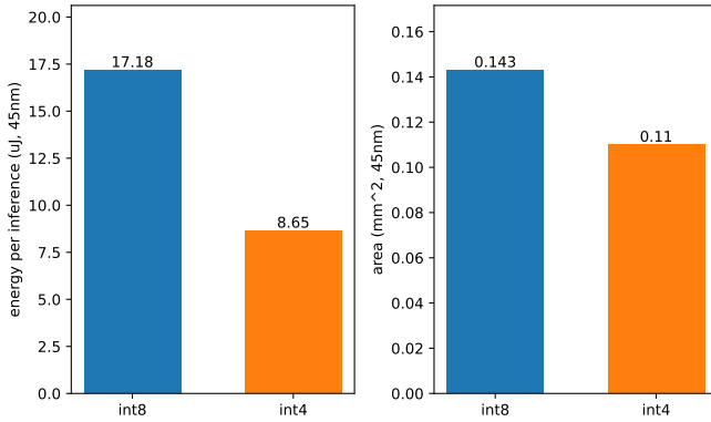
Fig. 5. int8 vs. int4 at the chosen design point: \sim 50\% energy and \sim 23\% area reduction (accuracy trade measured in Fig. 4).
