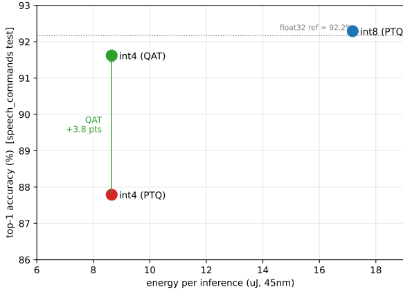
Fig. 4. Measured accuracy–energy trade on the MLPerf Tiny KWS test set: int4 weight quantization halves per-inference energy; post-training drops top-1 by \sim 4.5 points, but quantization-aware training recovers int4 to within \sim 1 point of float at the same energy.
