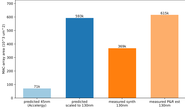
Fig. 7. Predicted (Acclergy 45 nm) vs. measured (Sky130 130 nm) MAC-array area; same order of magnitude after node and P&R correction.
