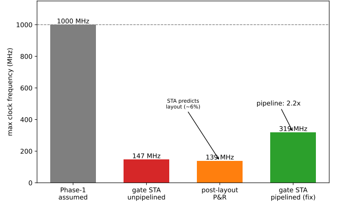
Fig. 6. Timing: the 1 GHz assumption is \sim 7\times optimistic; one pipeline stage recovers 2.2\times .
