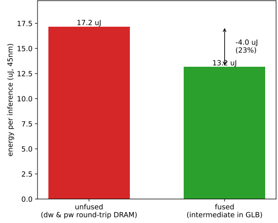
Fig. 3. Depthwise \rightarrow pointwise fusion keeps the intermediate activation on chip, cutting per-inference energy \sim 23\% .
