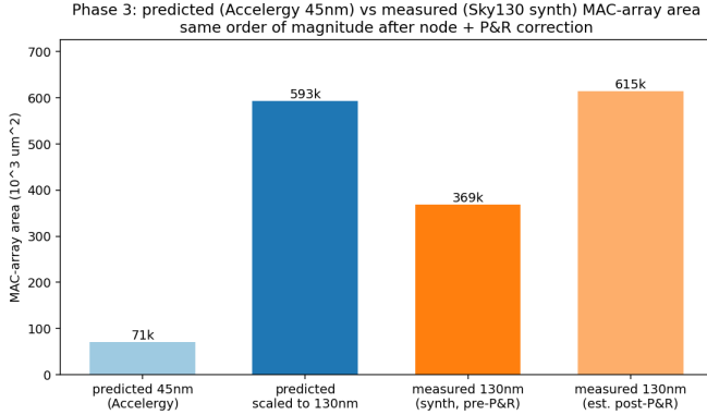
Fig. 7. Predicted (Accelergy 45 nm) vs. measured (Sky130 130 nm) MAC-array area; same order of magnitude after node and P&R correction.
