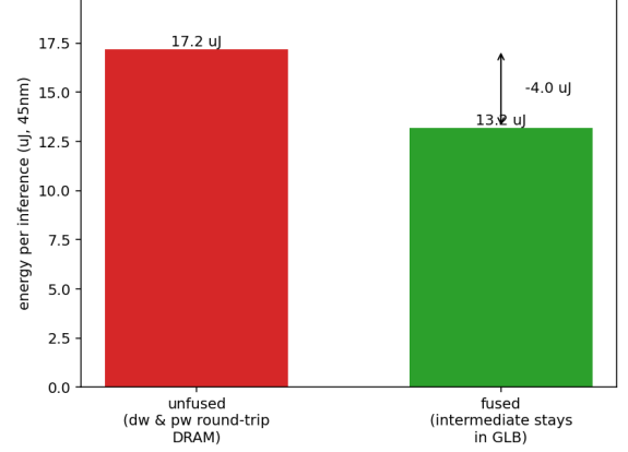
Depthwise→pointwise fusion: 23% energy cut (kills DRAM round-trip of the 8000-elem intermediate \times 4 blocks)
