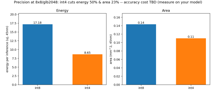
Fig. 4. int8 vs. int4 at the chosen design point: \sim 50\% energy and \sim 23\% area reduction (accuracy cost not evaluated here).
