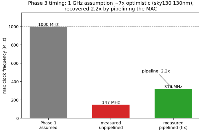
Fig. 5. Timing: the 1 GHz assumption is \sim 7\times optimistic; one pipeline stage recovers 2.2\times .
