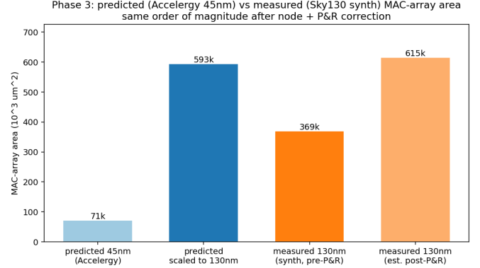
Fig. 6. Predicted (Accelergy 45 nm) vs. measured (Sky130 130 nm) MAC-array area; same order of magnitude after node and P&R correction.
