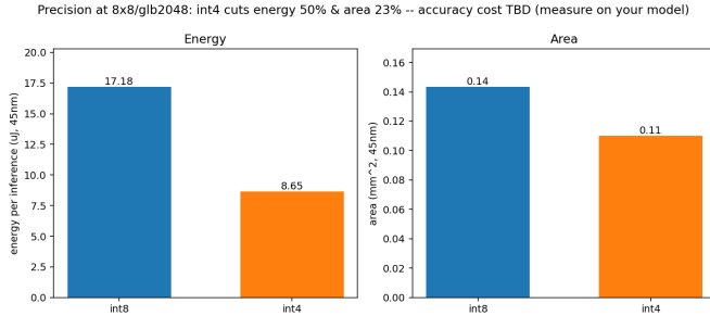
Fig. 5. int8 vs. int4 at the chosen design point: \sim 50\% energy and \sim 23\% area reduction (accuracy cost not evaluated here).
