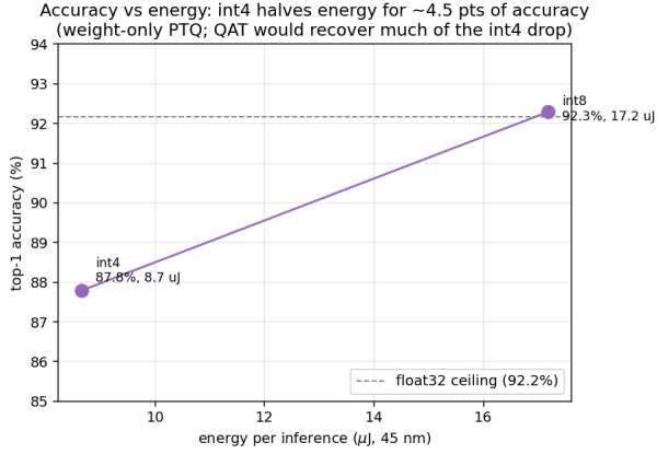
Fig. 4. Measured accuracy–energy trade on the MLPerf Tiny KWS test set: int4 weight quantization halves per-inference energy for a \sim 4.5 -point top-1 drop. Weight-only PTQ; quantization-aware training would recover much of it.
