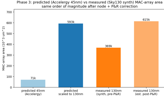
Fig. 7. Predicted (Accelergy 45 nm) vs. measured (Sky130 130 nm) MAC-array area; same order of magnitude after node and P&R correction.
