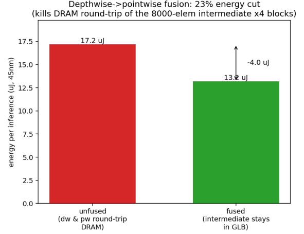
Fig. 3. Depthwise→pointwise fusion keeps the intermediate activation on chip, cutting per-inference energy \sim 23\% .
