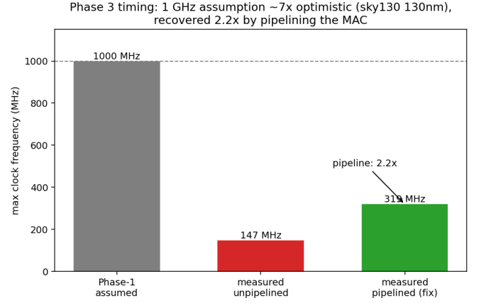
Fig. 6. Timing: the 1 GHz assumption is \sim 7\times optimistic; one pipeline stage recovers 2.2\times .
