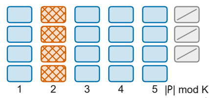
(f) Group CV+ (equal folds)
