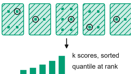
(e) Single subsampling (calibration)
