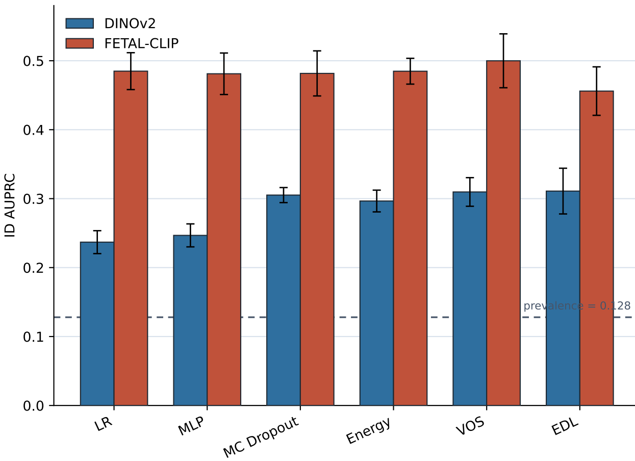
In-distribution classification
