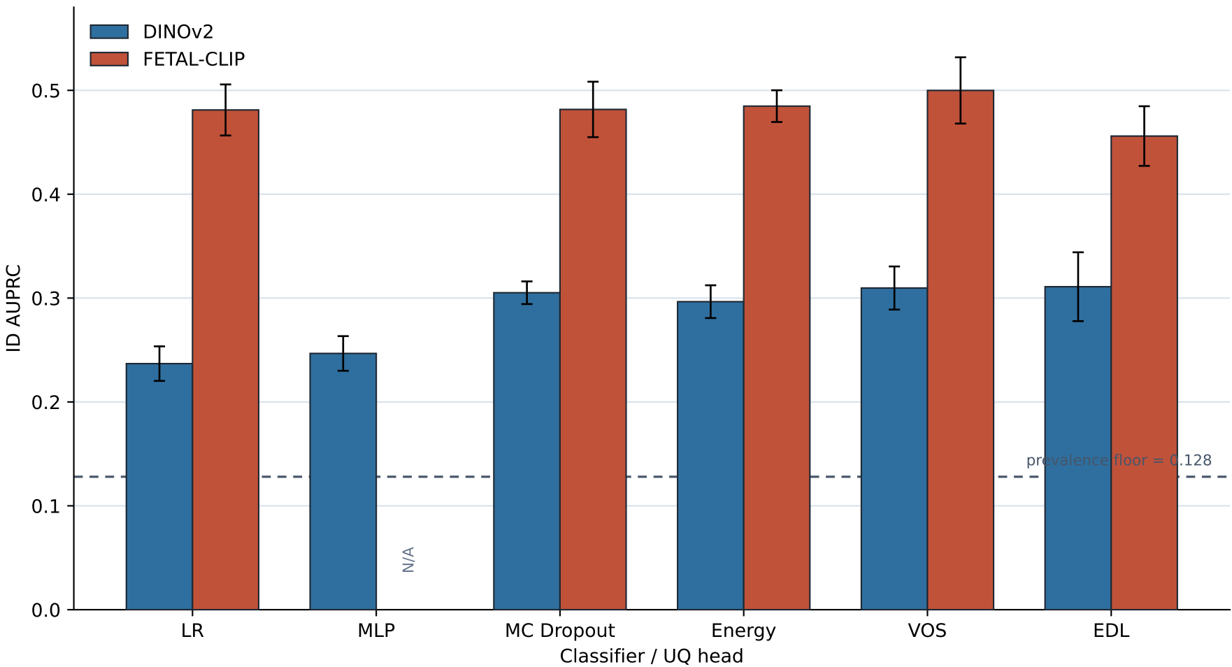
Encoder Lift in In-Distribution CHD Classification
