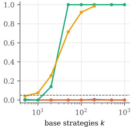
(c) DSR certifies, \rho = 0.3
