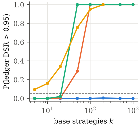
(b) DSR certifies, \rho = 0.0
