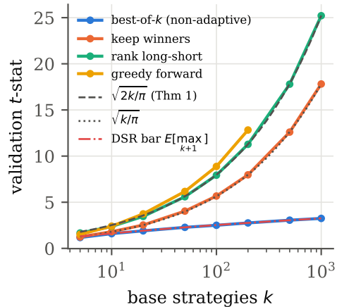
(a) validation t , \rho = 0
