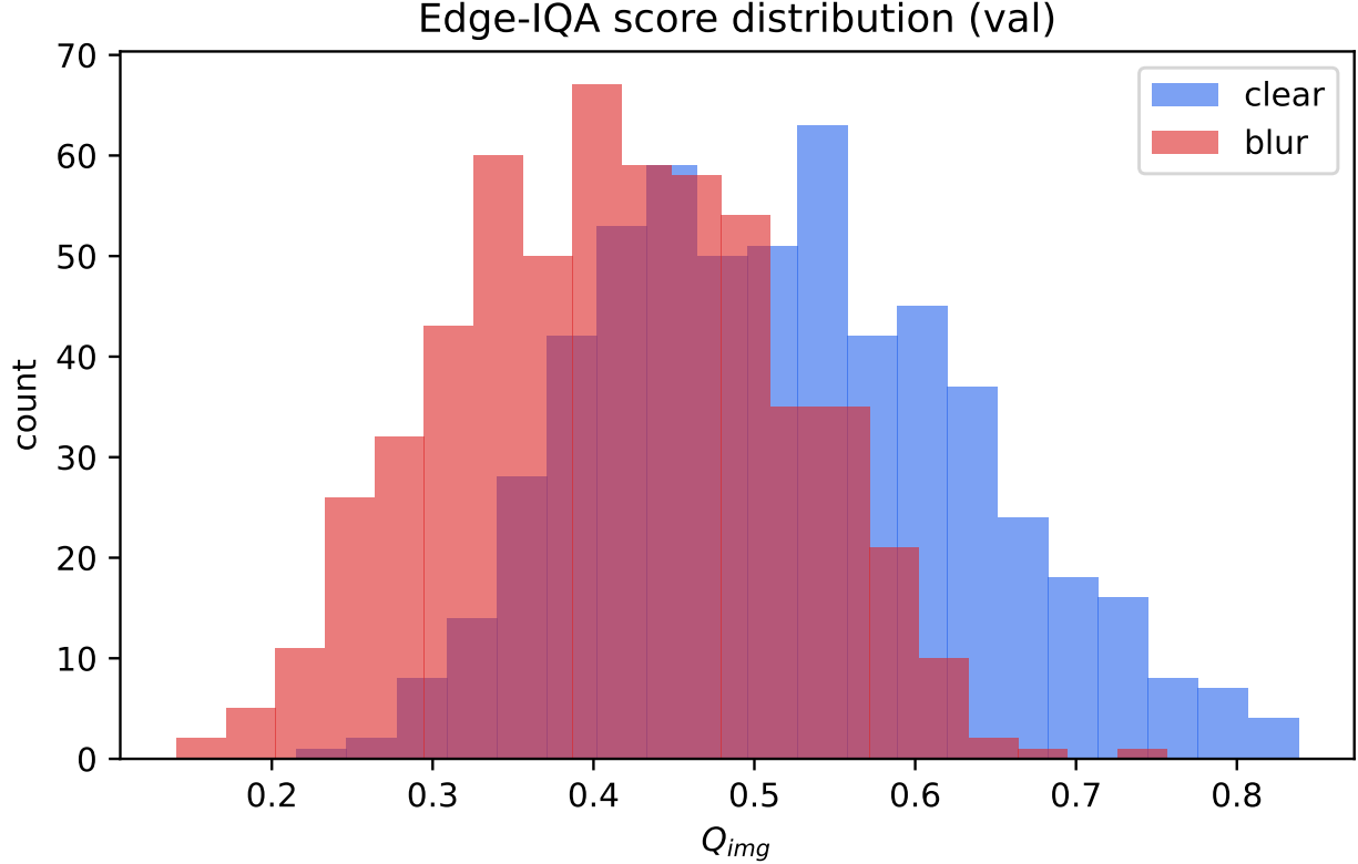
Figure 3: Edge-IQA Q_{img} on ShezhenV3 validation: clear vs. synthetically blurred pairs ( n=1,144 ).
