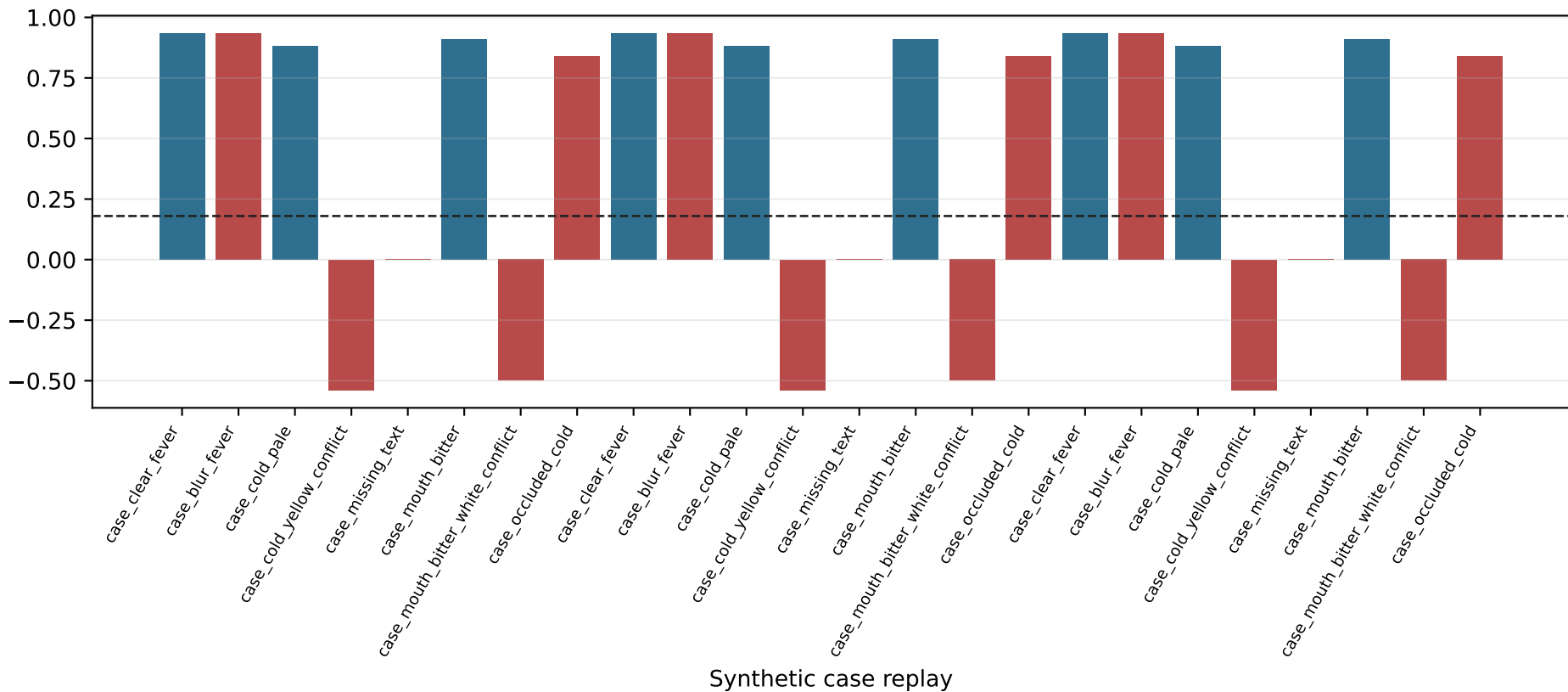
Embedding compatibility
