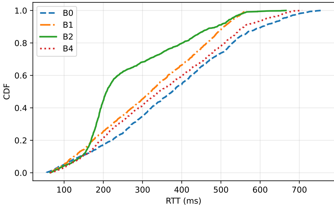
End-to-end RTT (offline main experiment)
