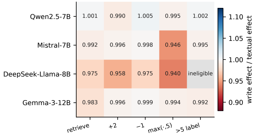
a Consequence matching across families
