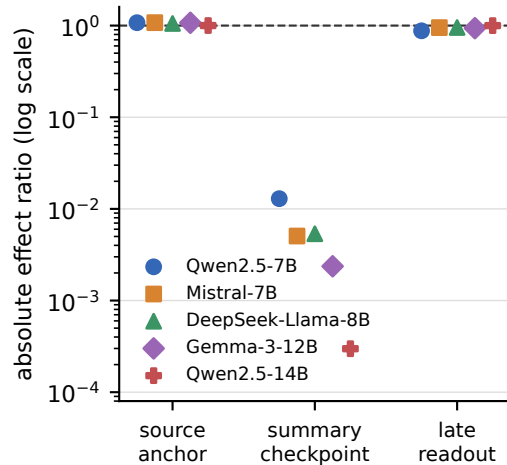
b Anchor-checkpoint-readout contrast
