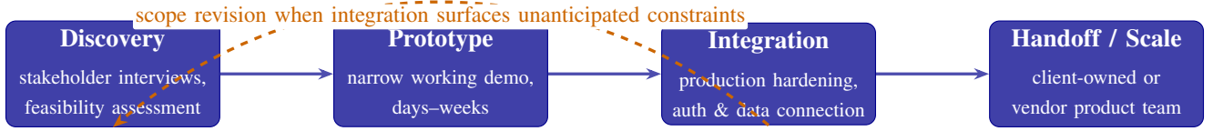
Fig. 1. The FDE engagement lifecycle. Discovery, Prototype, Integration, and Handoff/Scale form the main sequence (solid arrows); the dashed feedback arrow denotes the common case in which integration-stage findings force a return to Discovery, a loop that flat, sequentially-budgeted engagement plans do not account for.
