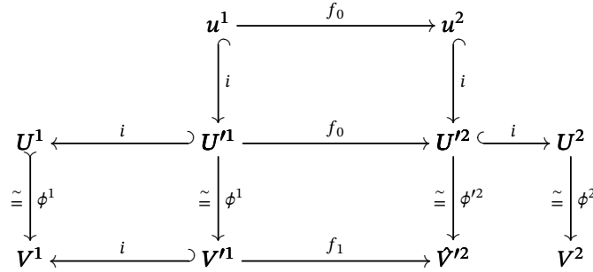
Figure 4: Completed m-atlas morphism
