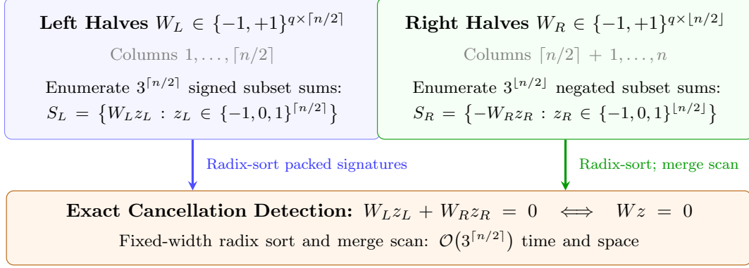
Figure 3: Meet-in-the-middle ternary kernel counter using fixed-width radix sorting and a merge scan for cancelling signatures.
