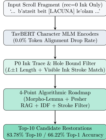
Figure 1: System Architecture: End-to-end pipeline combining character TavBERT MLM, physical P_0 ink filtering, and the 4-point roadmap.
