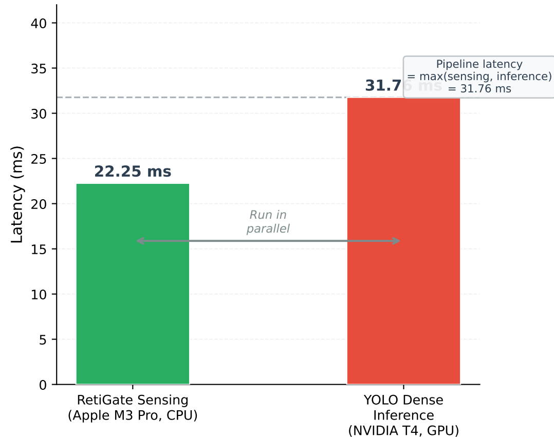
Sensing vs Inference Latency (separate hardware, pipelined)
