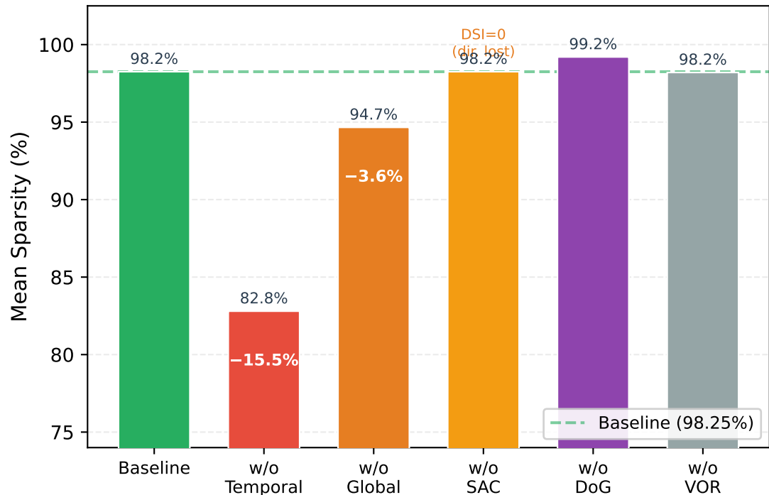
Ablation Study
