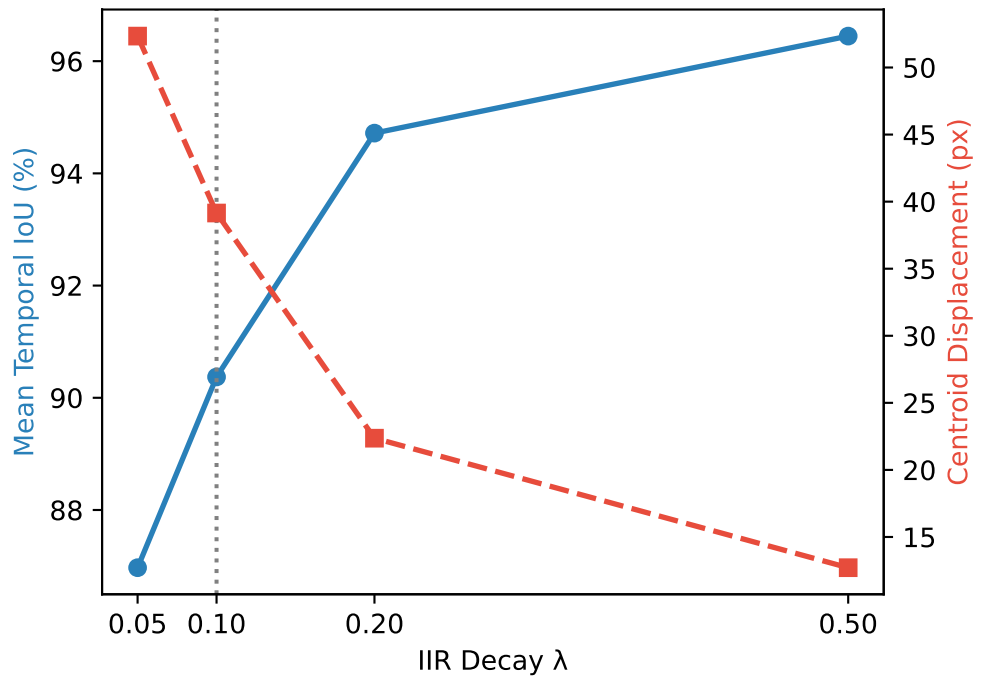
\lambda Effect on Temporal Stability
