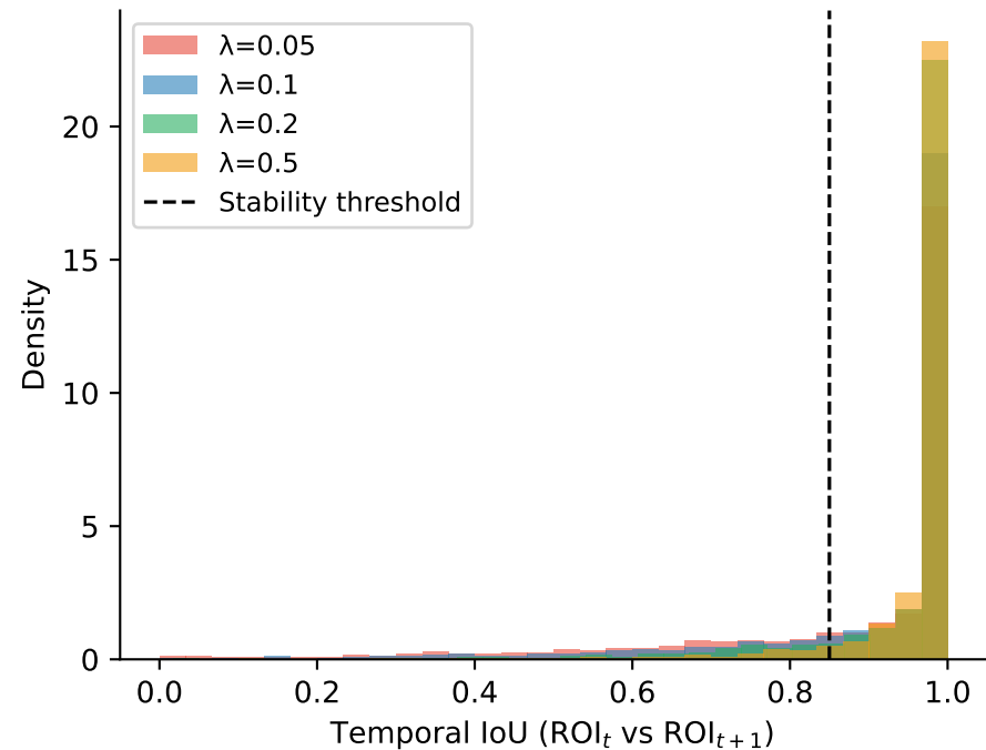
ROI Temporal Stability by IIR \lambda
