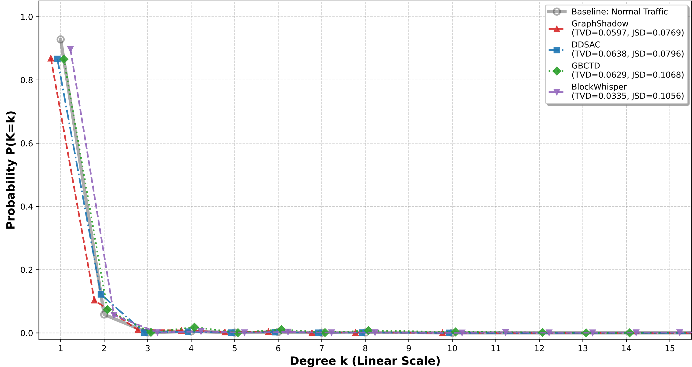
Degree Distribution Comparison & Quantified Similarity
