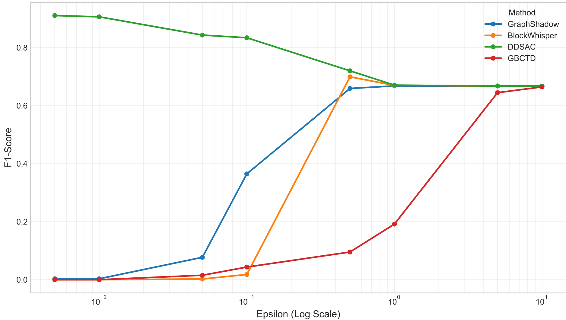
F1-Score vs Epsilon (Fixed Quota)
