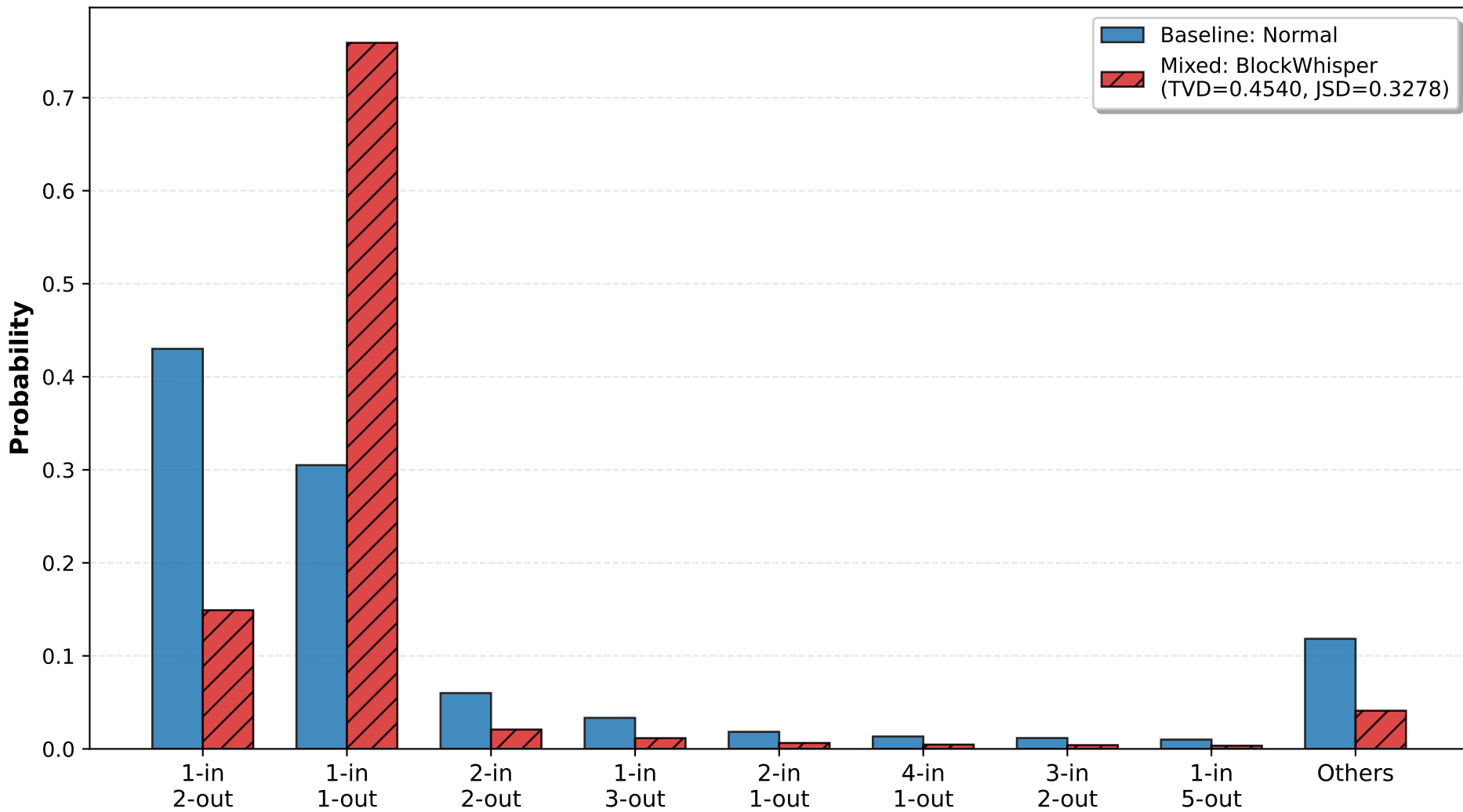
Transaction Structure Distribution (BlockWhisper)
