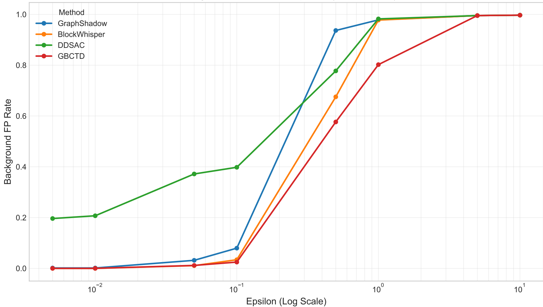
Background FP Rate vs Epsilon (Fixed Quota)
