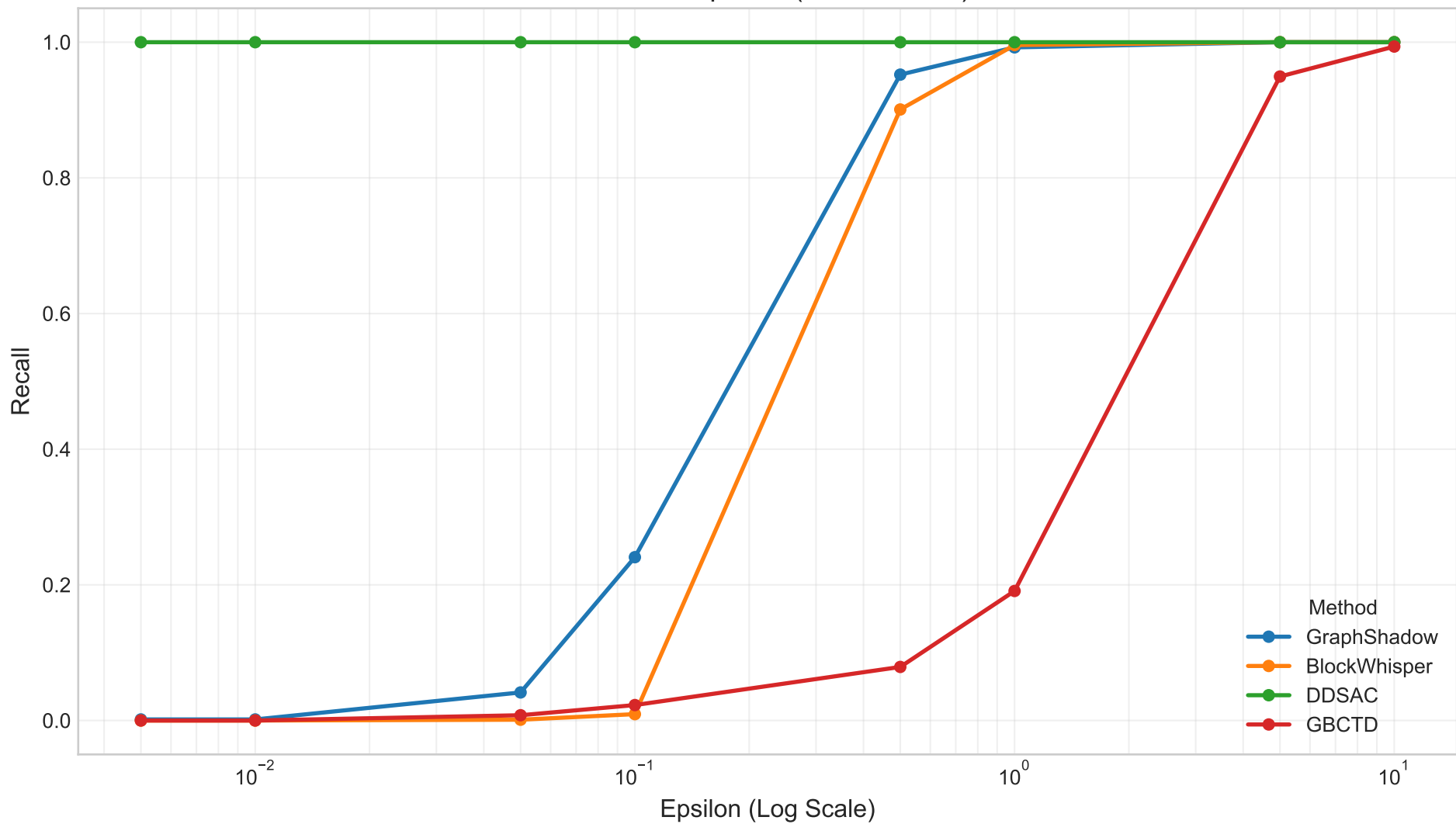
Recall vs Epsilon (Fixed Quota)
