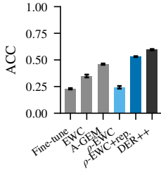
(b) Split-CIFAR-100 (task-IL)
