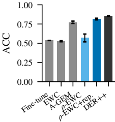
(a) Split-CIFAR-10 (task-IL)
