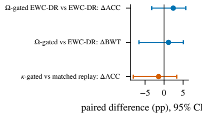
(c) Gated sign tests
