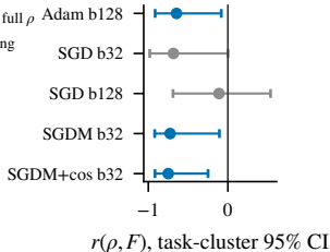
(c) Optimizer regime
