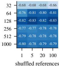
(a) Estimator grid, r(\rho, F)
