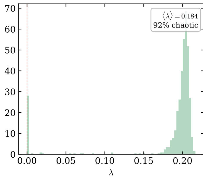
(c) Stadium FTLE, \alpha = 0.5
