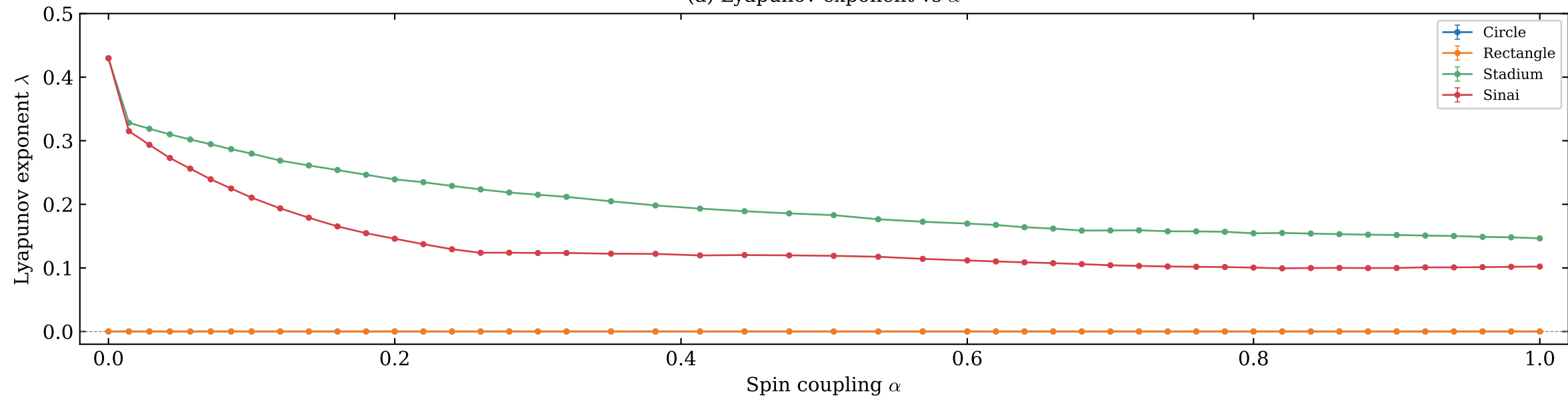
(a) Lyapunov exponent vs \alpha
