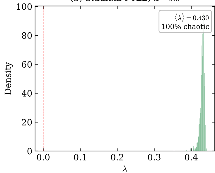
(b) Stadium FTLE, \alpha = 0.0
