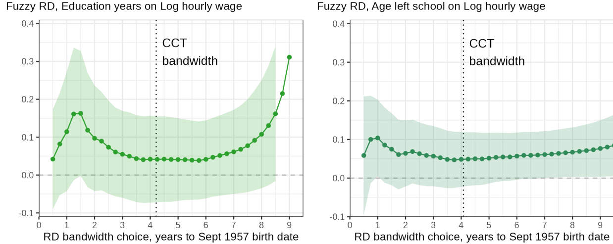
Figure A3: Fuzzy RDD Estimates, Sensitivity to Bandwidth Choice.
