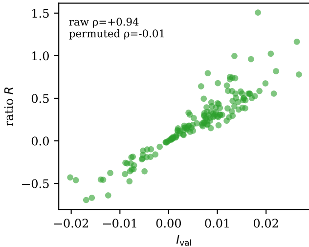
(b) ratio leakage
