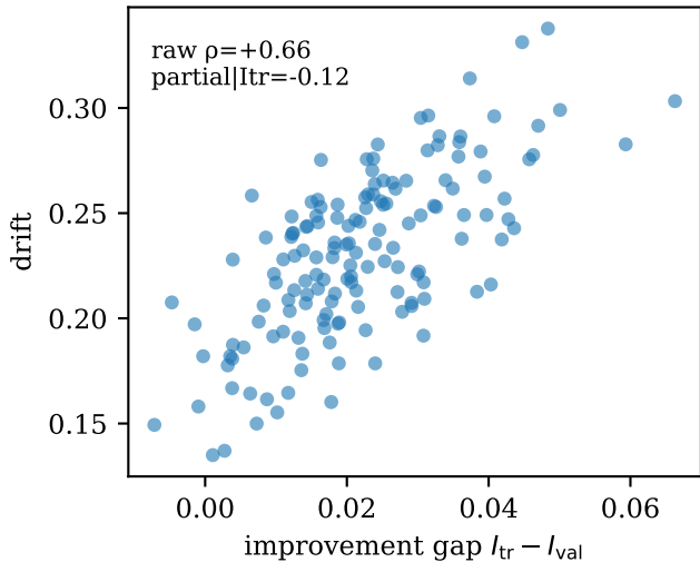
(a) drift coupling
