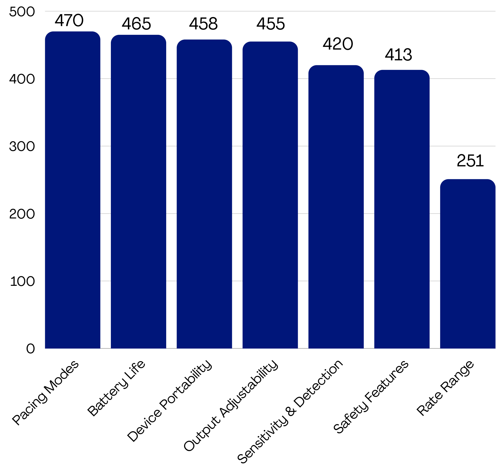
Aspect Distribution
