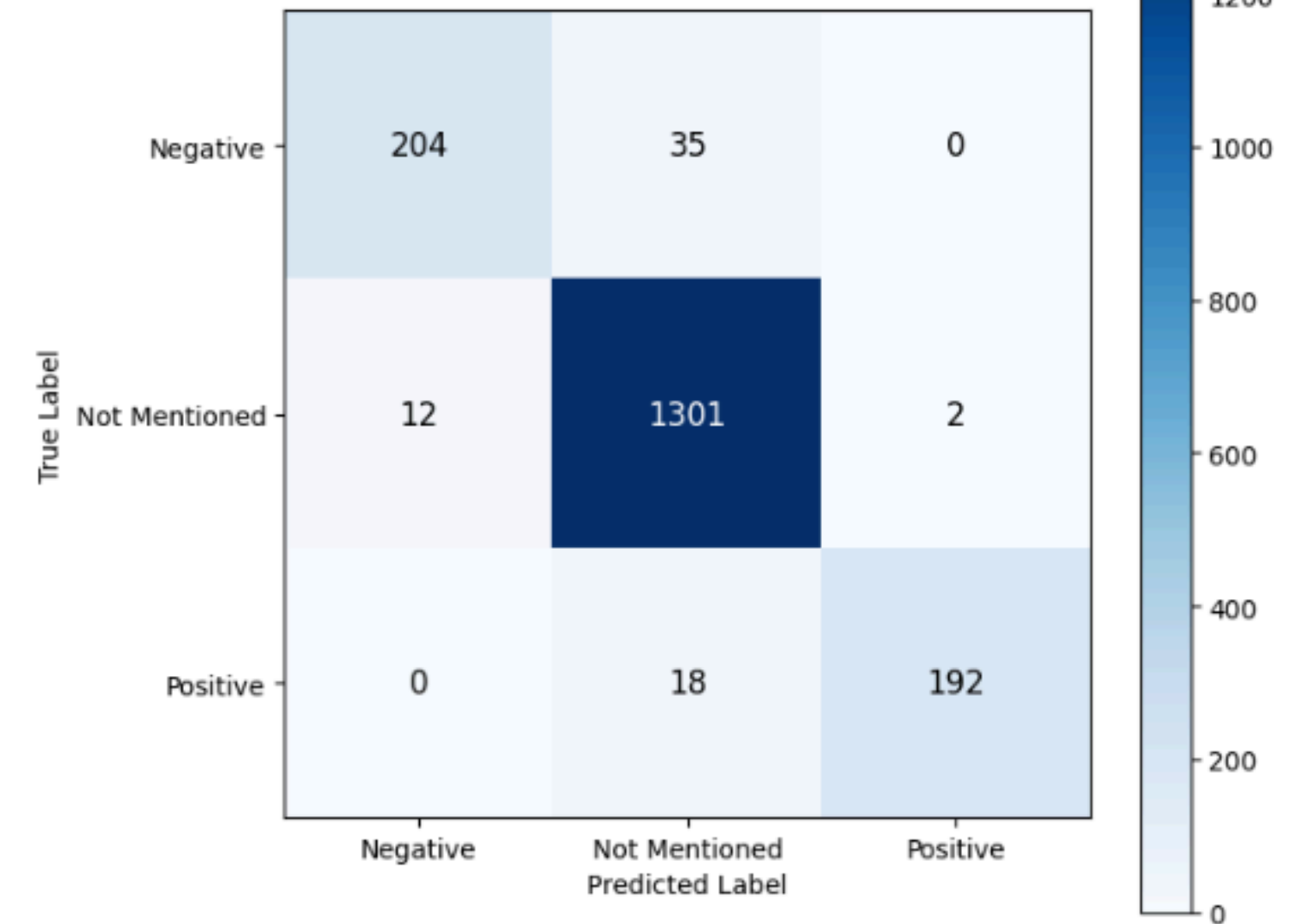
Confusion Matrix
