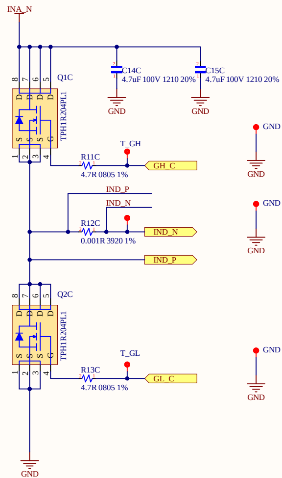
3-Phase Half Bridge
