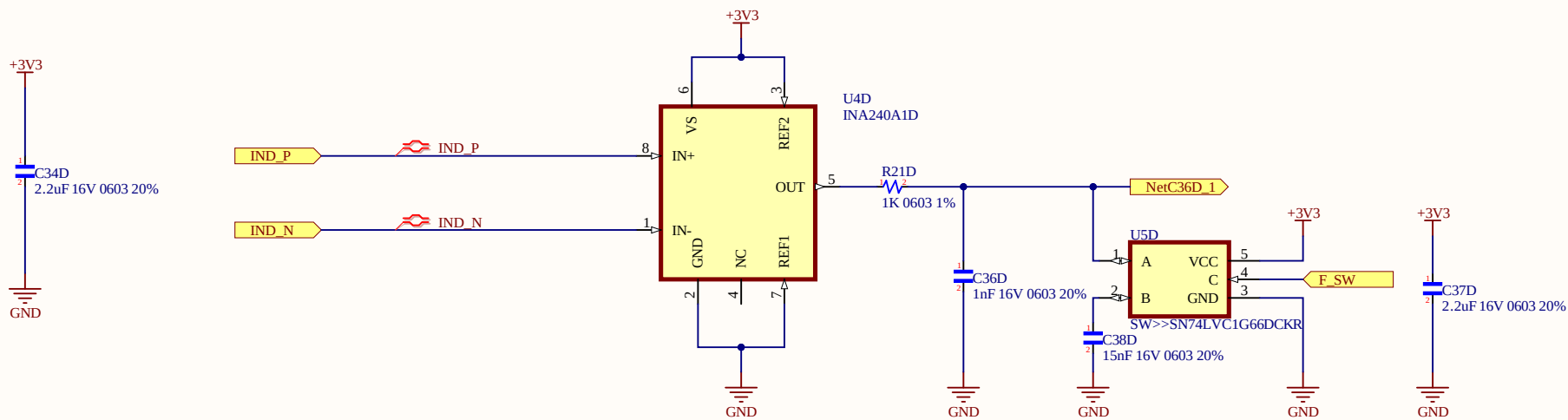
Current Shunt Amplifier
