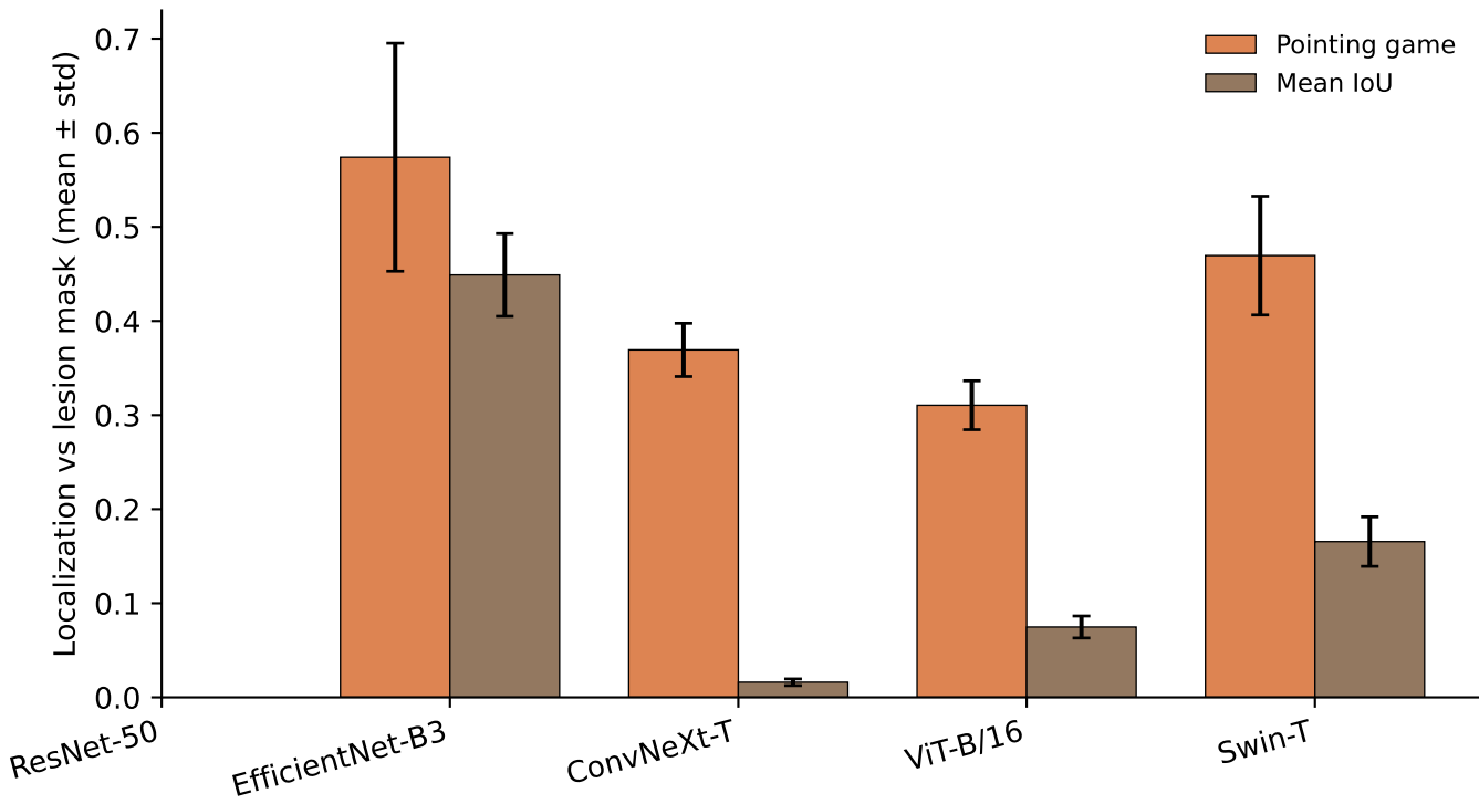
Lesion localization of Grad-CAM++ explanations
