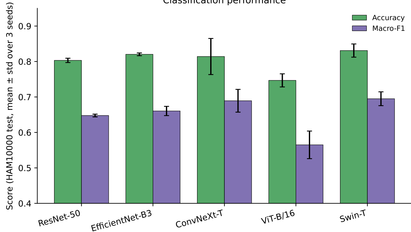
Classification performance
