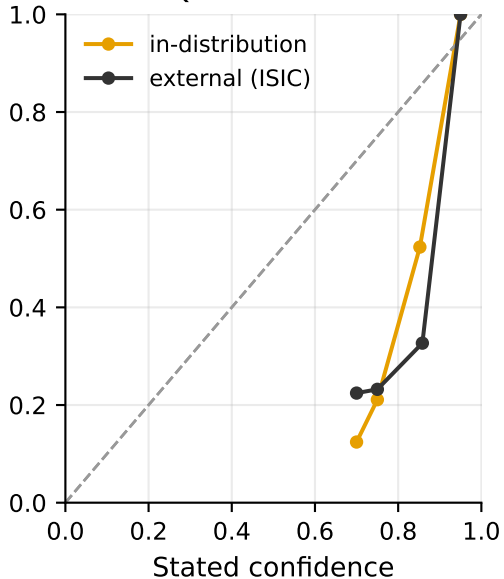
Qwen3.5-0.8B
