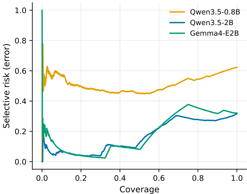
Risk-coverage (HAM test, A_v1)
