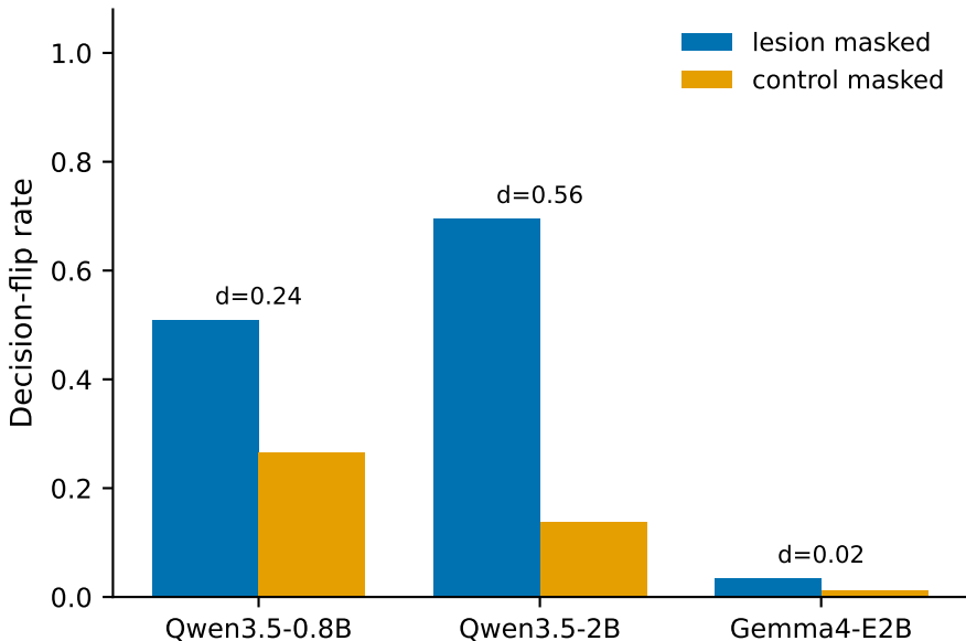
Faithfulness: flips under lesion vs control masking
