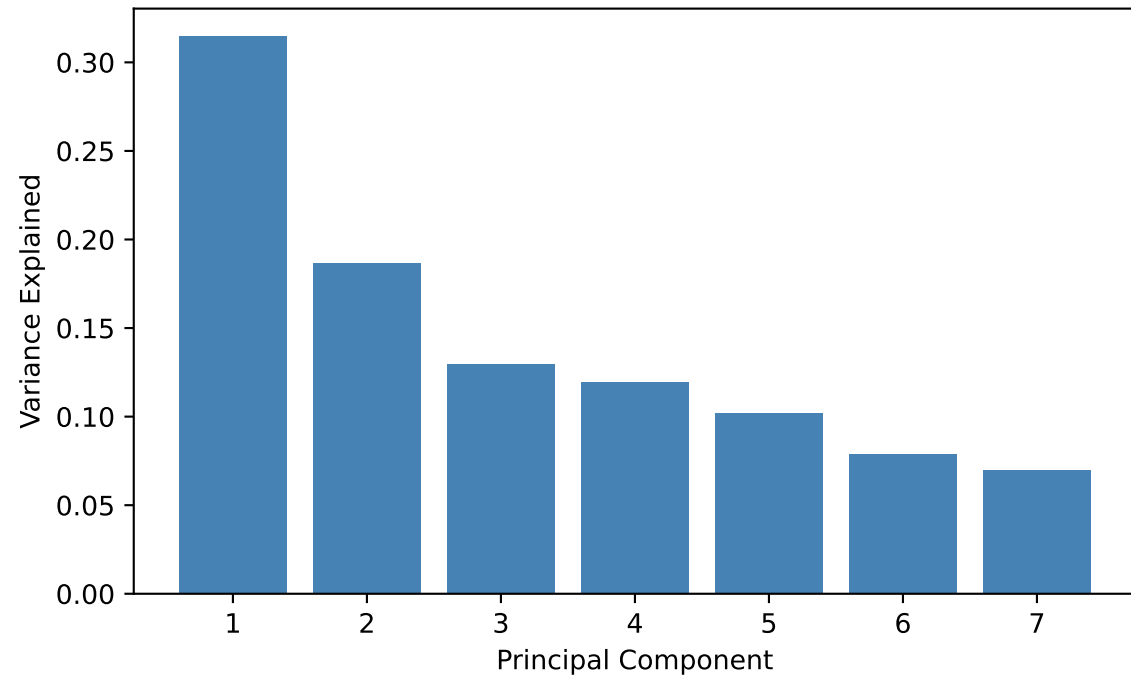
Scree Plot
