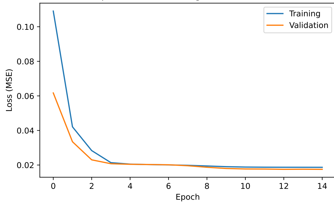
Output from the training of an autoencoder
